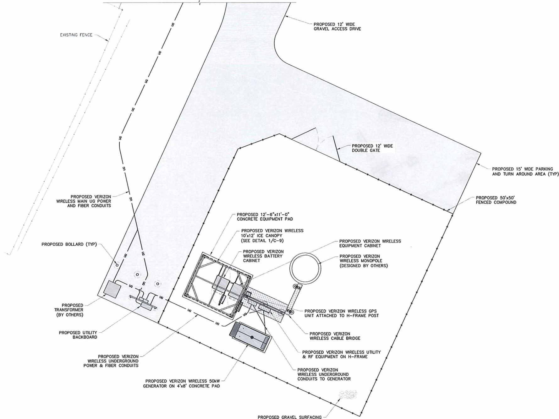
1 C-2 SITE DETAIL PLAN SCALE: 1" = 10' (11x17 SIZE) 1" = 5' (22x34 SIZE)
